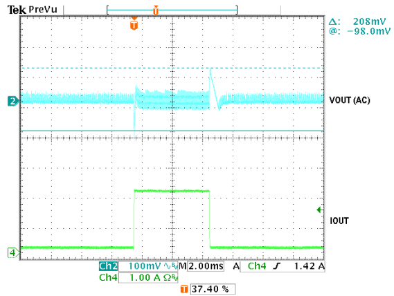
Load Transient (VIN=40V, VOUT=5V, Load=0.1~2A)
