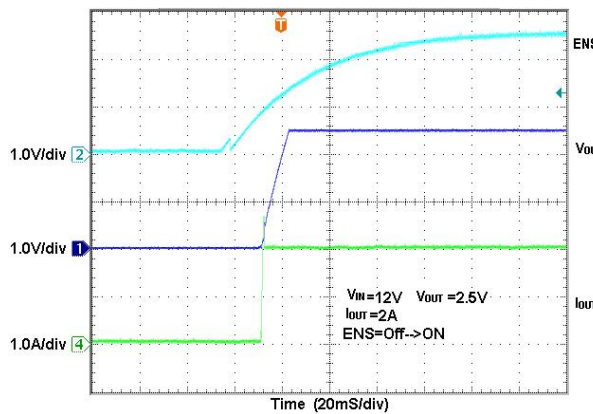
Enable-ON Wave ( V_{IN}=12V , V_{OUT}=2.5V , Load=2A, C_{EN}=0.1\mu F )
