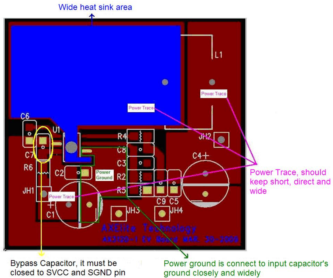
(AX3120A SOP-8L-EP PCB Layout -Top View)
