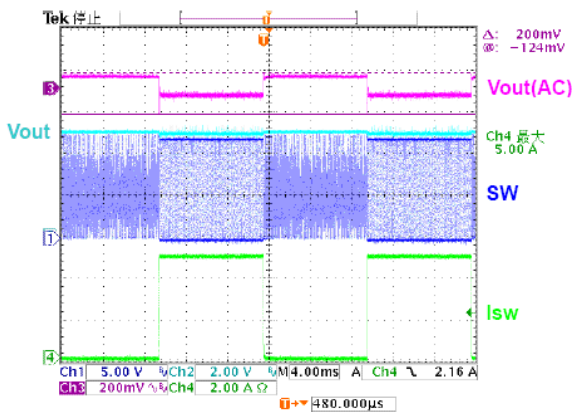
Output Ripple ( V_{IN}=12V, V_{OUT}=5V, I_{OUT}=5A )
