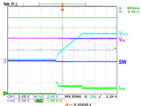
Start-Up from Thermal Shutdown ( V_{IN}=12V, V_{OUT}=5V, I_{OUT}=1A )
