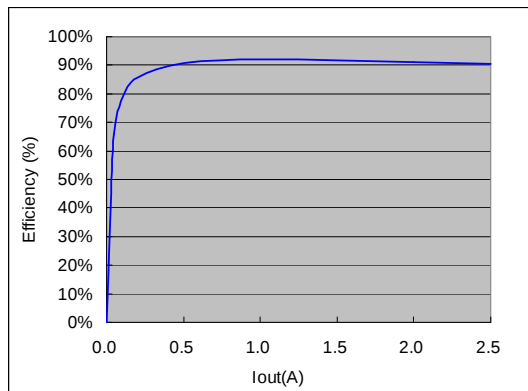
Efficiency ( V_{IN}=12V , V_{OUT}=5V )
