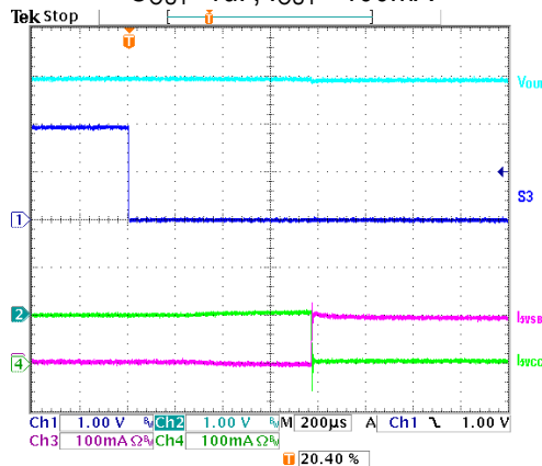
S3# High to Low C OUT =1uF, I OUT =100mA
