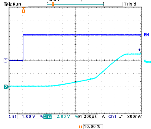
Turn On into 5VCC C OUT =1uF, S3#=5V
