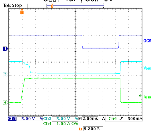
OCP for 5VSB C OUT =1uF, S3#=0V
