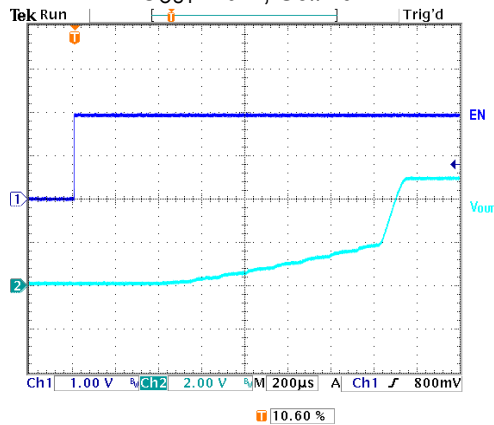
Turn On into 5VSB C OUT =1uF, S3#=0V
