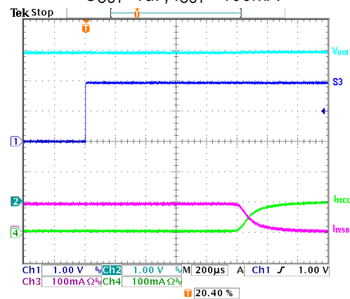
S3# Low to High C OUT =1uF, I OUT =100mA
