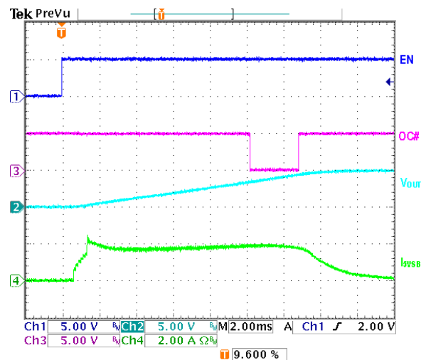
Figure1. Turn on into 5V SB with 5000µF output capacitor.
