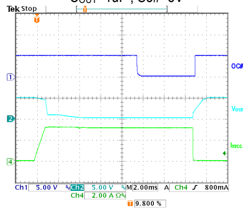
OCP for 5VCC C OUT =1uF, S3#=5V
