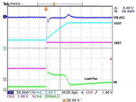
Load Transient (VIN Drop)
