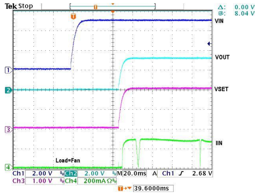
Fully-On
