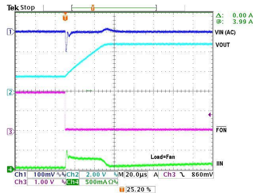
Load Transient (VIN Drop)
