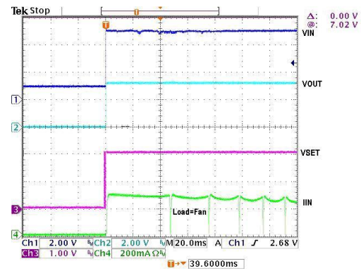
Fully-On(VIN Drop)
