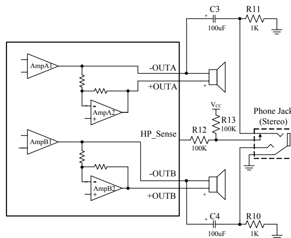
Figure 2. Headphone Circuit
