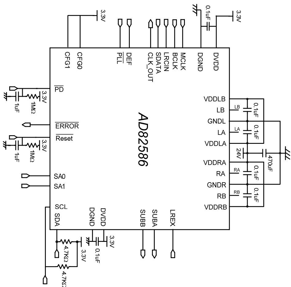
Application Circuit Example for stereo with subwoofer PWM output
