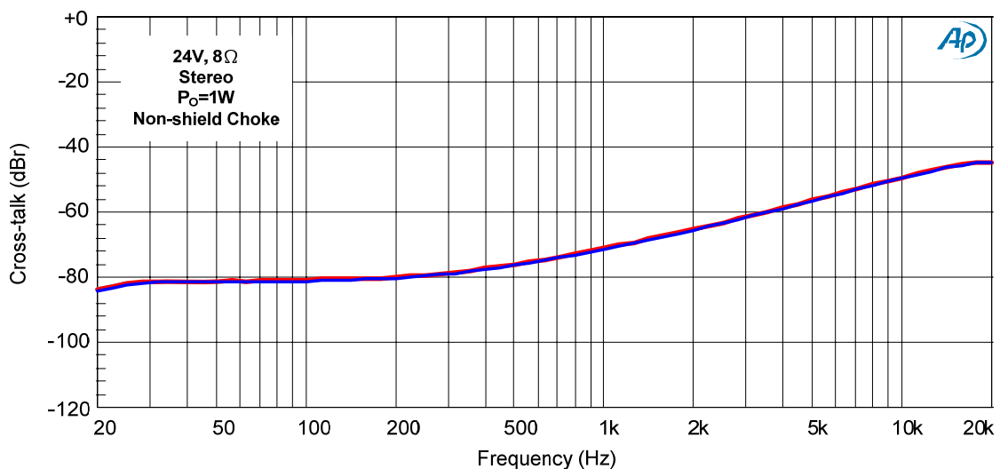
Cross-talk (Stereo)
