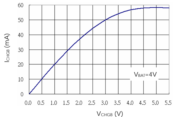
CHGB Pin I-V Curve (Strong Pull-Down State)
