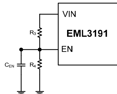
Fig.16 Two external resistors on EN pin
