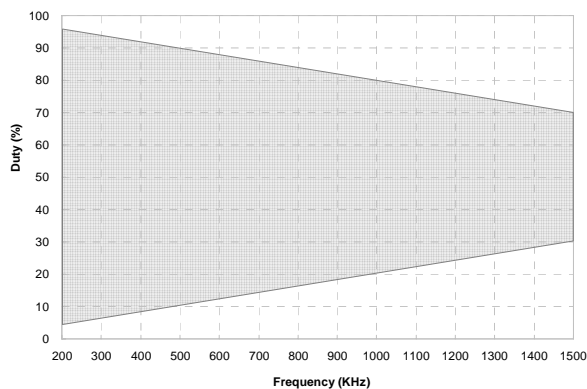
Fig.15 EML3191 Safe Operating Voltage Area
