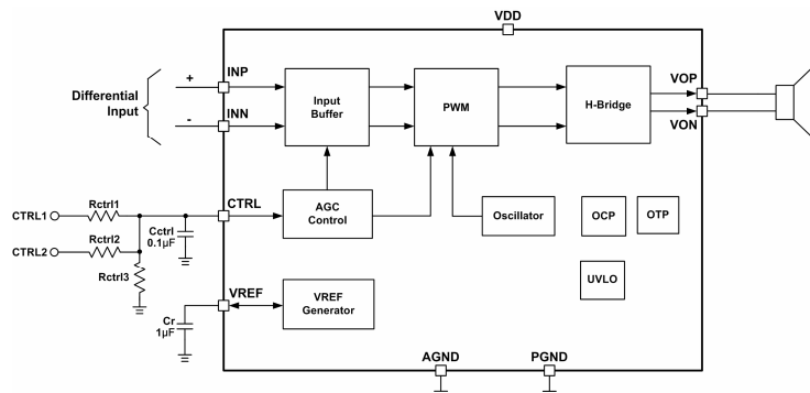
Figure 29. Differential Input Configuration
