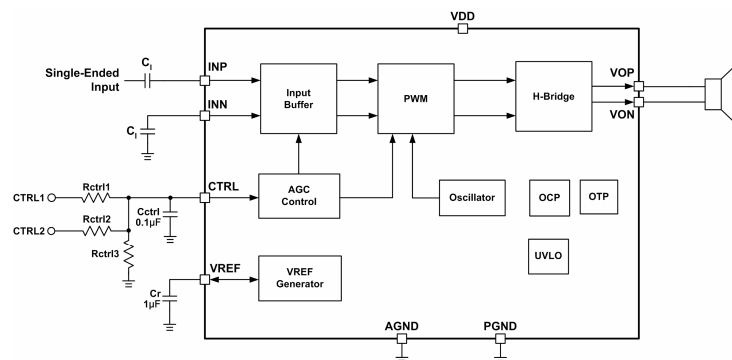
Figure 31. Single-Ended Input Configuration
