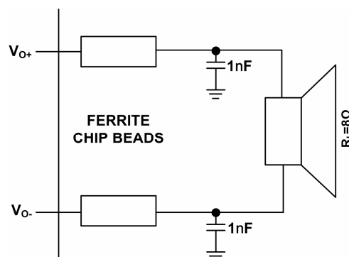
Figure 36. Optional EMI Ferrite Bead Filter
