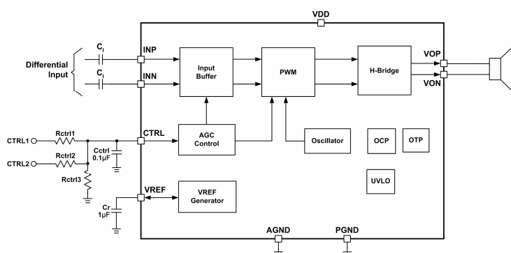
Figure 30. Differential Input Configuration and Input Capacitors
