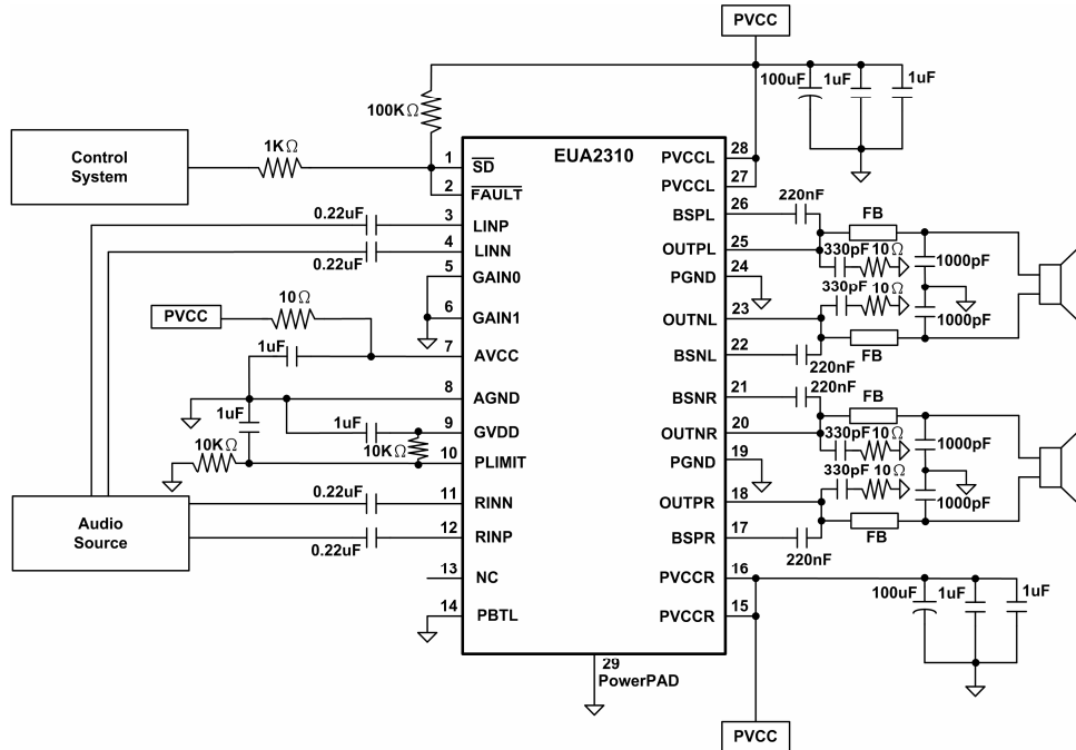
Figure 38. Differential Input
