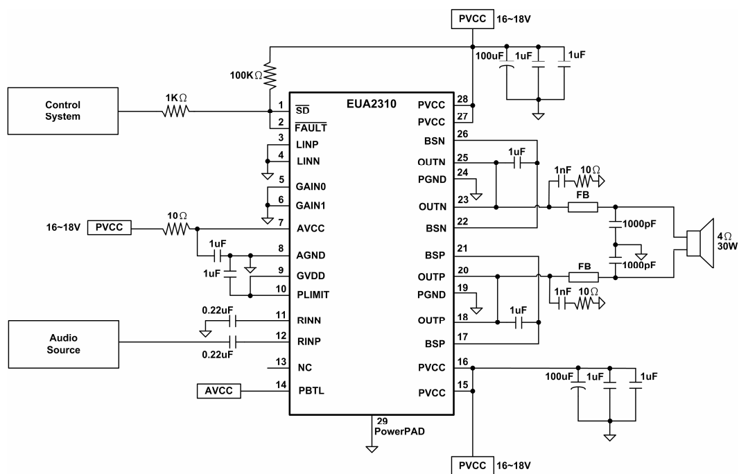
Figure 40. 4Ω/30W PBTTL Output
