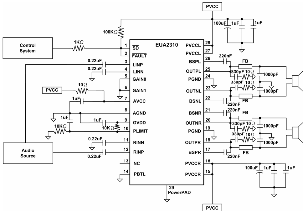
Figure 39. Single Ended Input
