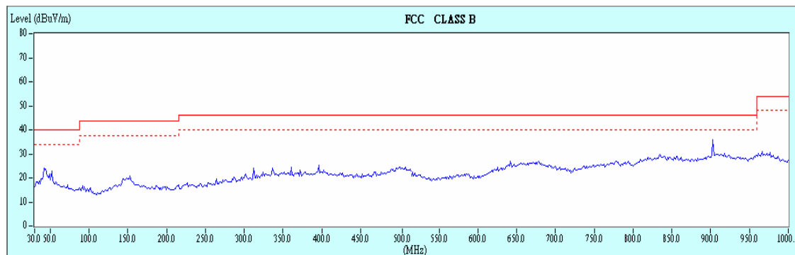
Figure37. EMI Test and FCC Limits
