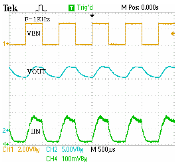
V_{IN}=3.6V Driving 6LEDs 1KHz PWM Dimming
