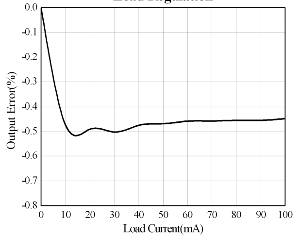
Positive Charge-Pump Regulator Load Regulation
