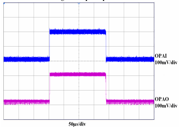
Operational Amplifier Small-signal Step Response
