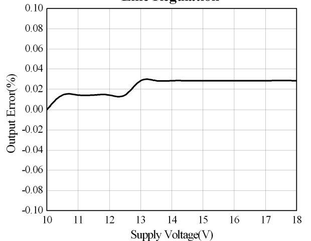
Negative Charge-Pump Regulator Line Regulation
