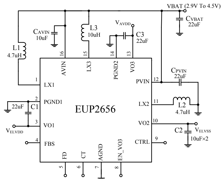
Figure 1. Application Circuit
