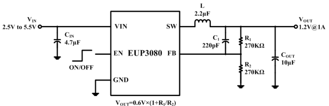
Figure 1. Application Circuit
