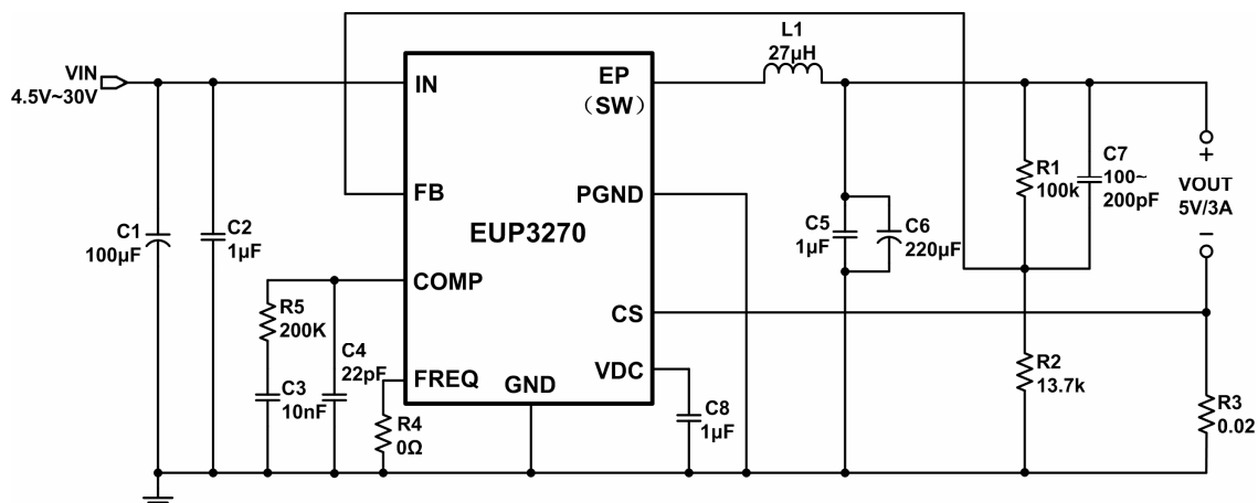
Figure 1. 150KHz Operating Frequency Application Circuit
