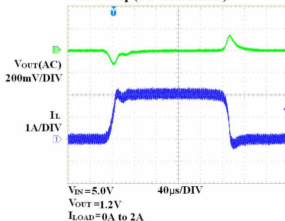
Load Step(FPWM Mode)
