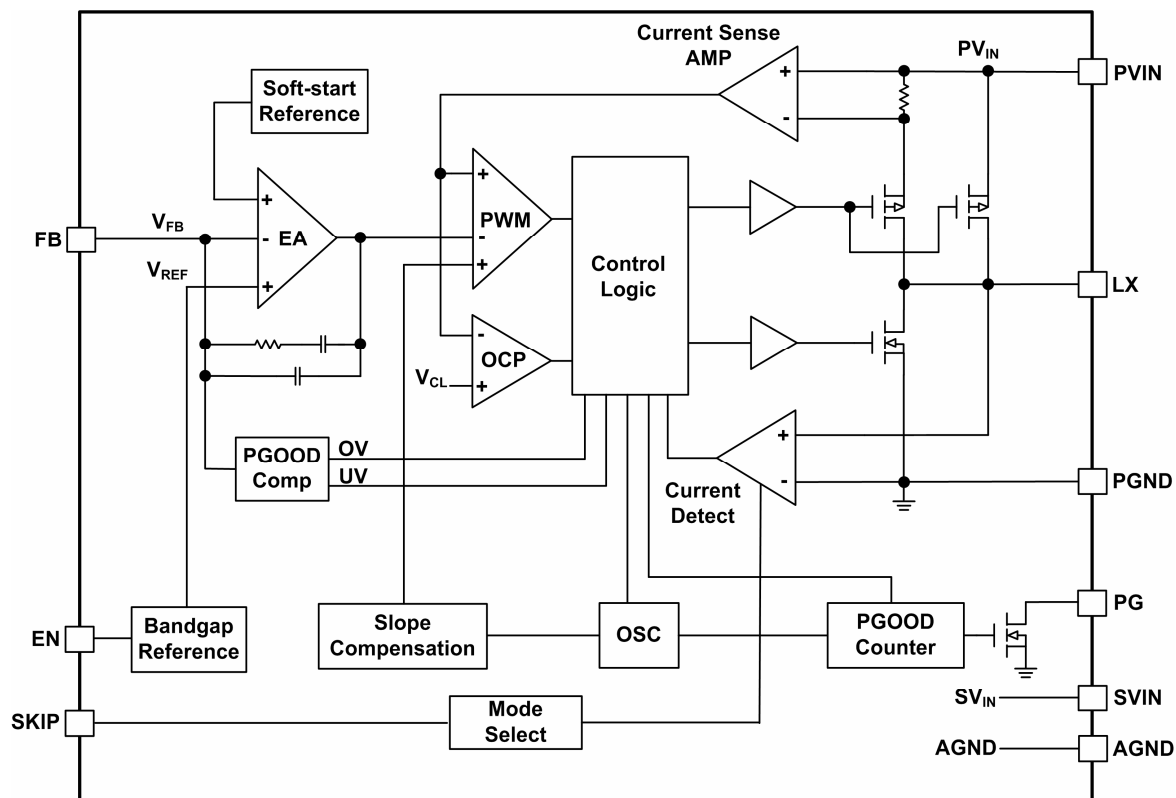
Figure3. Block Diagram
