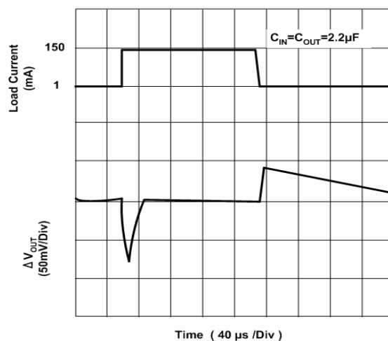
Load Transient Response ( V_{IN}=3.2V )
