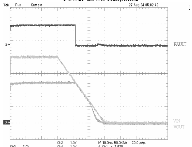
Power-down Response
