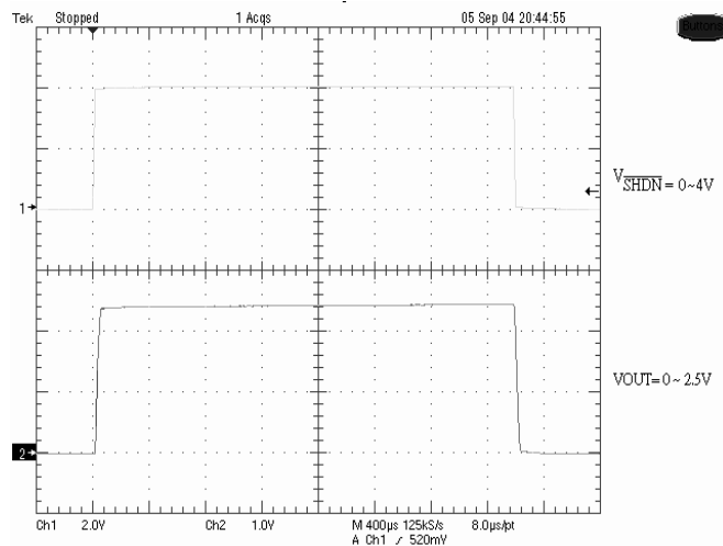
Shutdown Response
