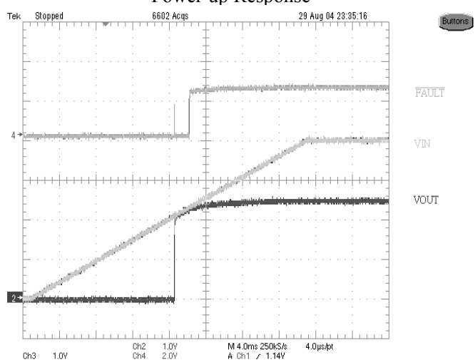
Power-up Response
