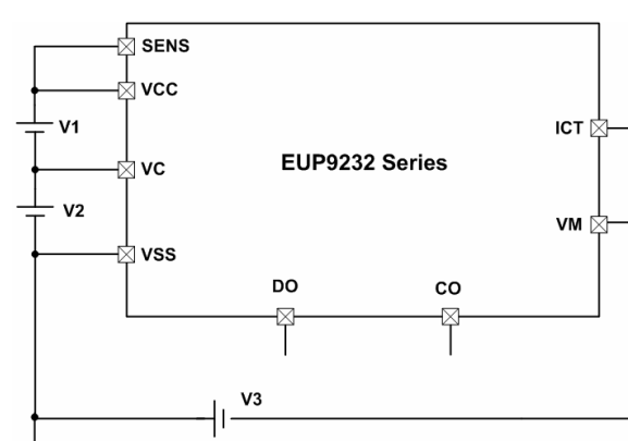
Test Circuit 6
