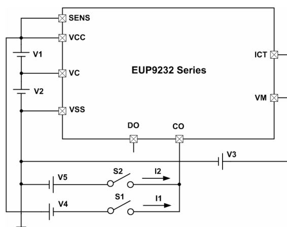
Test Circuit 4
