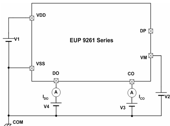
Measurement Circuit 4
