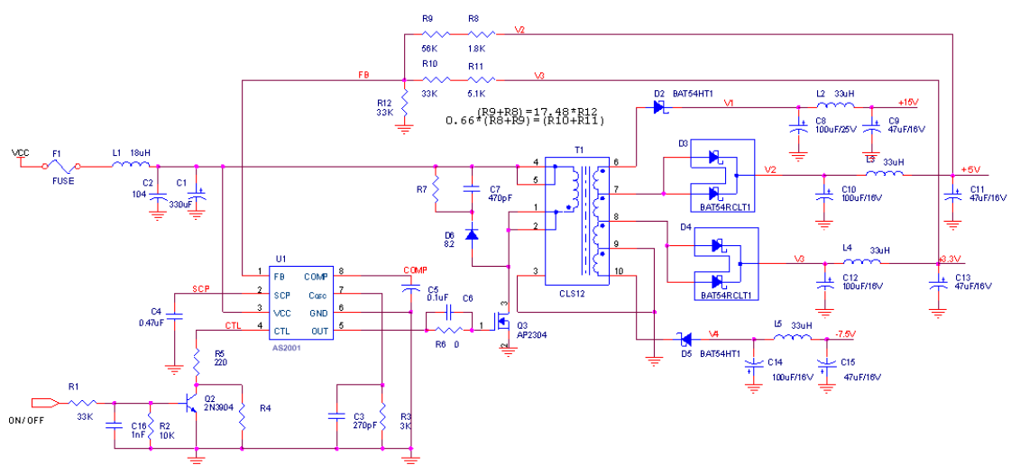
Figure17 Flyback Multi-Output DC-DC Converter Circuit
