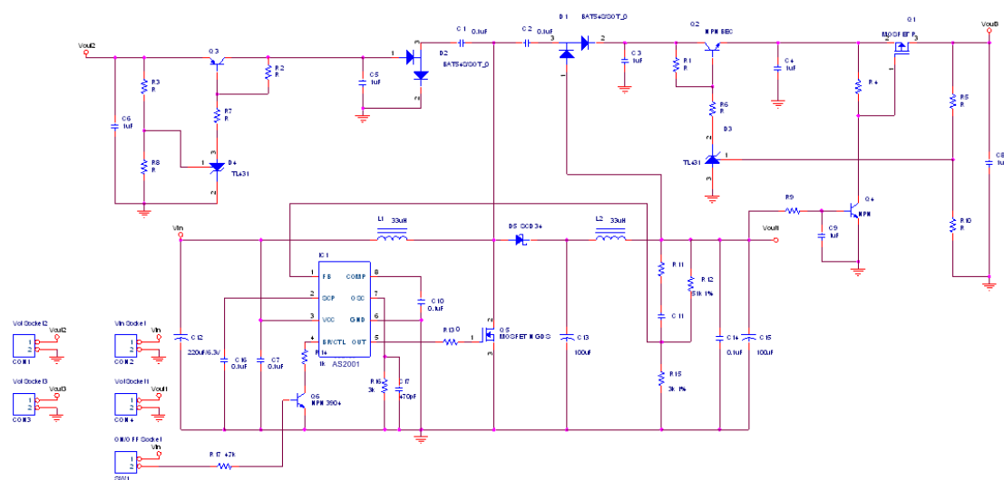
Figure16 Charge Pump DC-DC Converter Circuit
