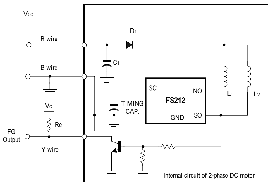
Fig 9 Application Circuit
