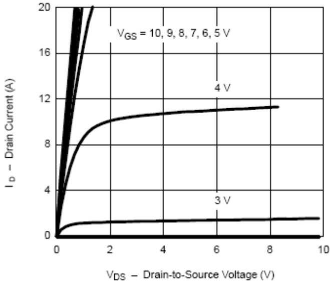
Output Characteristics
